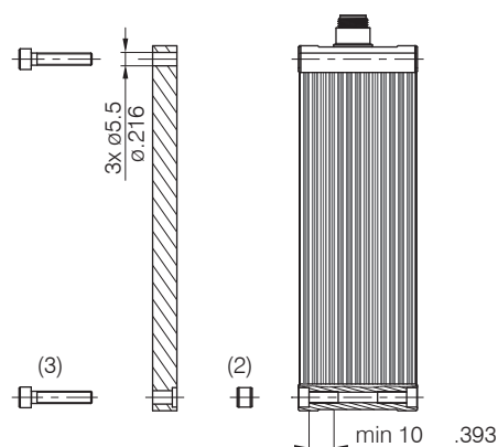
Fig. 6 Mounting example with direct fastening
