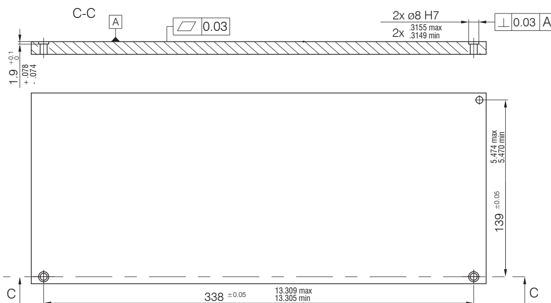
Fig. 8 Dimensional drawing mounting bores, sensor surfaceCONTROL 3D 35xx-240, dimensions in mm (inches, rounded off)
