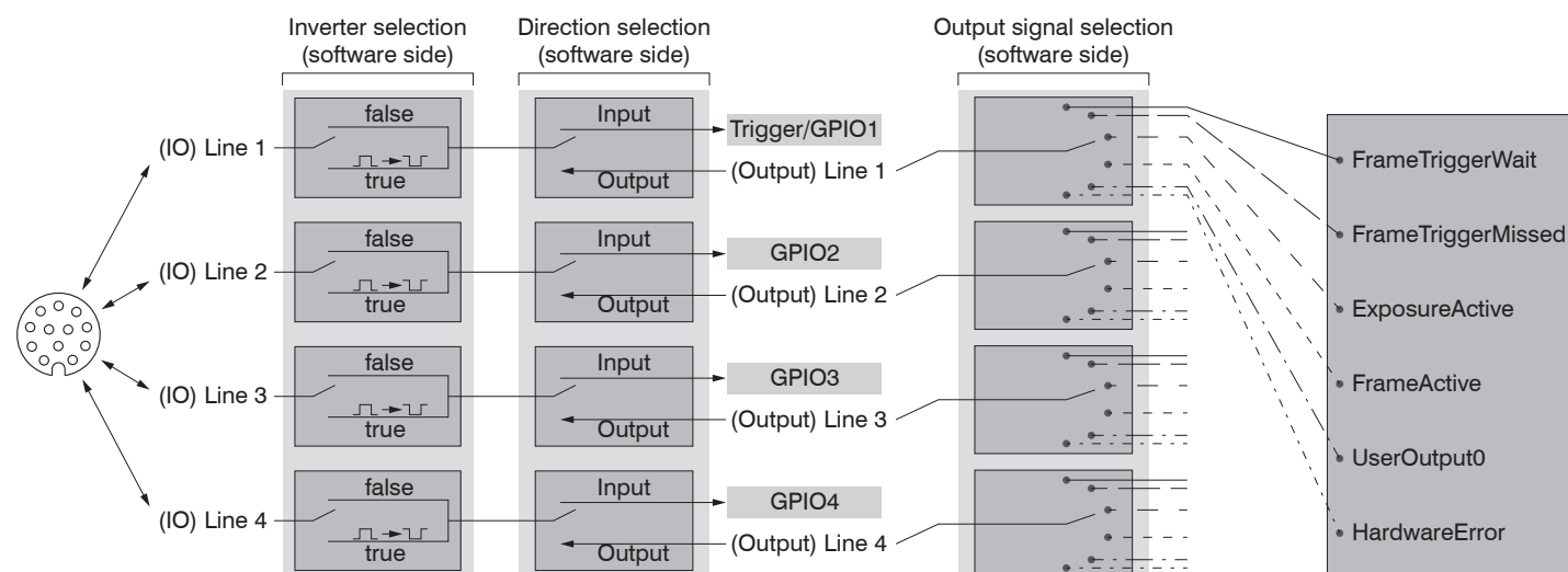
Fig. 17 Programmable inputs and outputs
