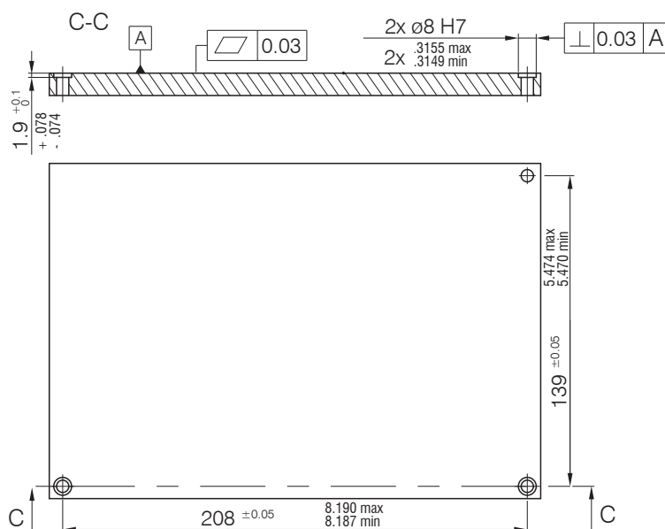
Fig. 7 Dimensional drawing mounting bores, sensor surfaceCONTROL 3D 35xx-80 und surfaceCONTROL 3D 32xx-120, dimensions in mm, not to scale (inches, rounded off)
