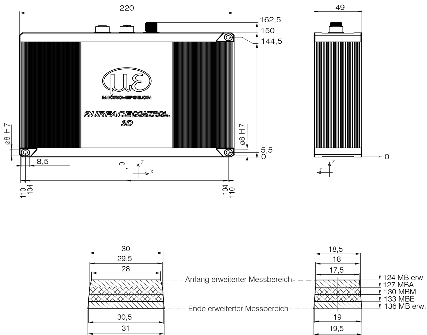
Fig. 9 Dimensional drawing sensor surfaceCONTROL 3D 35xx-30, dimensions in mm (inches, rounded off)
