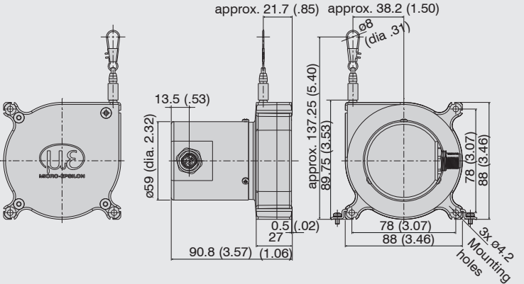
Dimensions drawing WPS-XXXX-MK88 with CANopen and connector M12, dimensions in mm (inches, rounded off)
