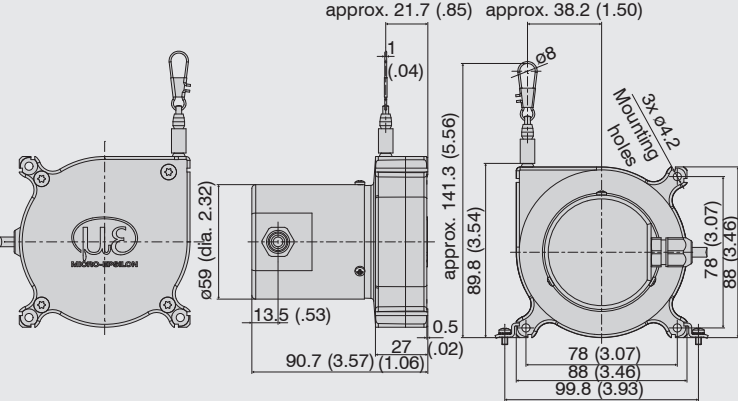
Dimensional drawing WPS-XXXX-MK88 with potentiometer, voltage, current and integrated cable, dimensions in mm (inches, rounded off)
